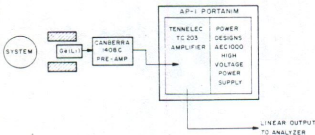
Fig. 2. Block diagram, passive gamma-ray system.
